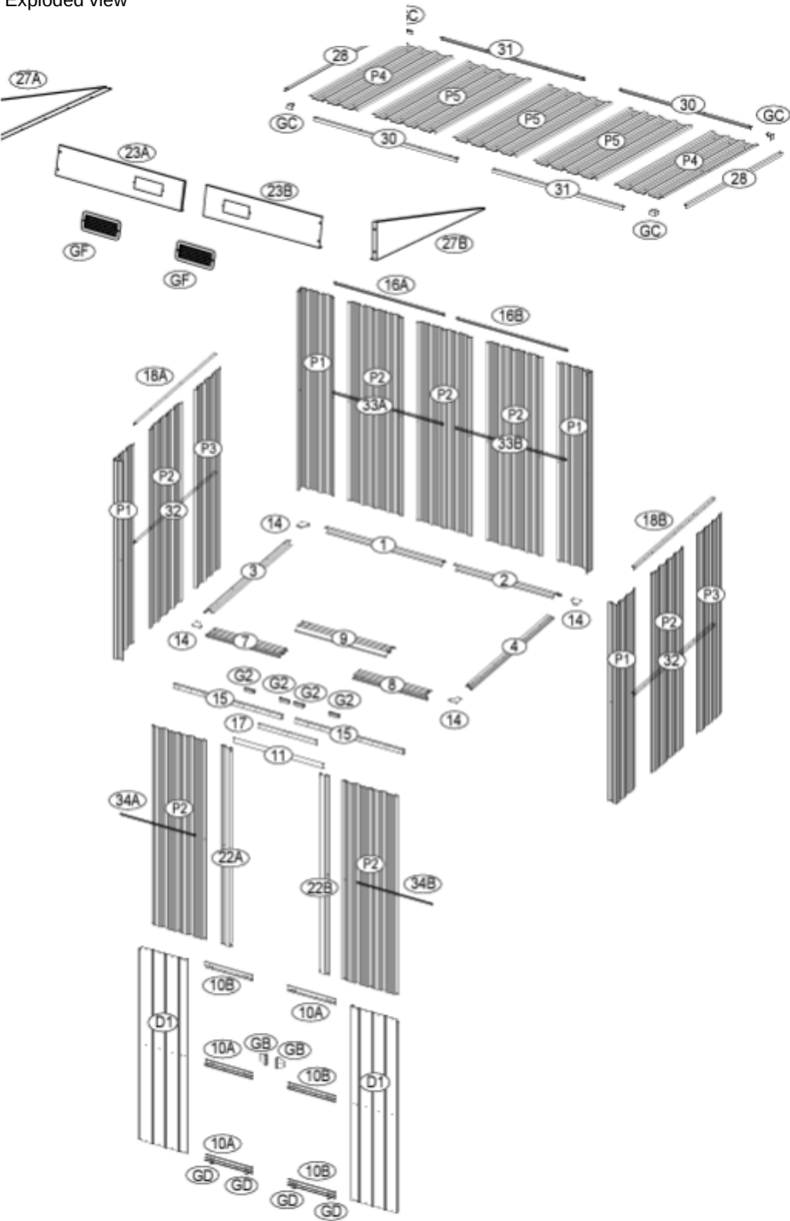
Exploded view
