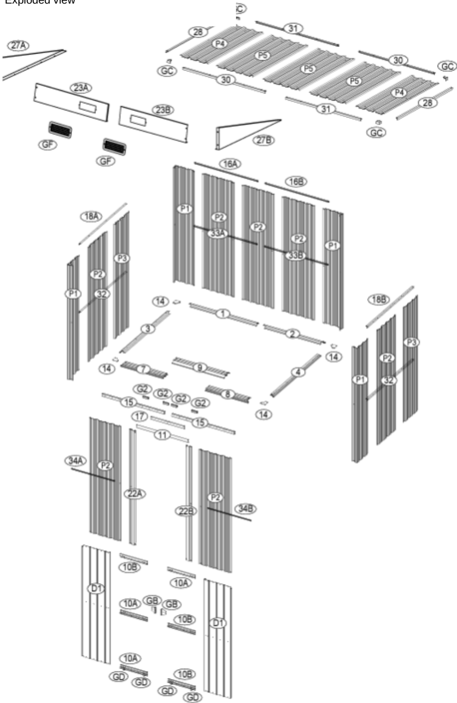
Exploded view
