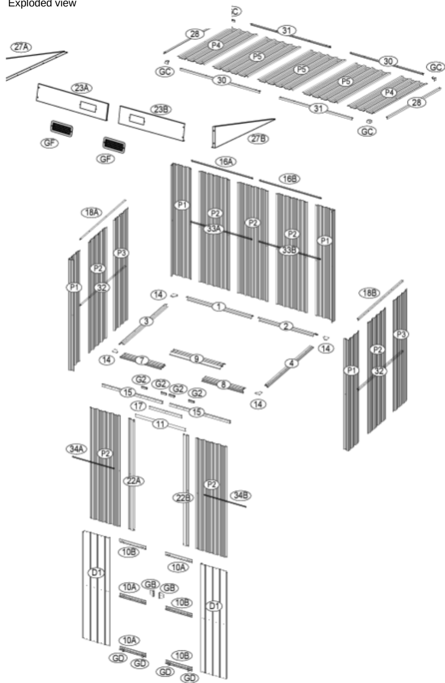
Exploded view
